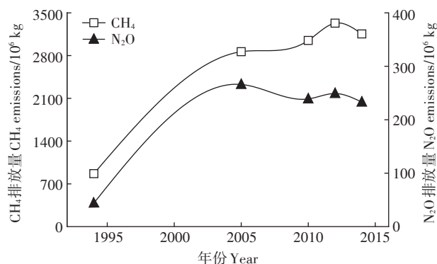
图1 中国5次畜禽粪便管理温室气体排放清单 Figure 1 Five greenhouse gas inventories for manure management in China
